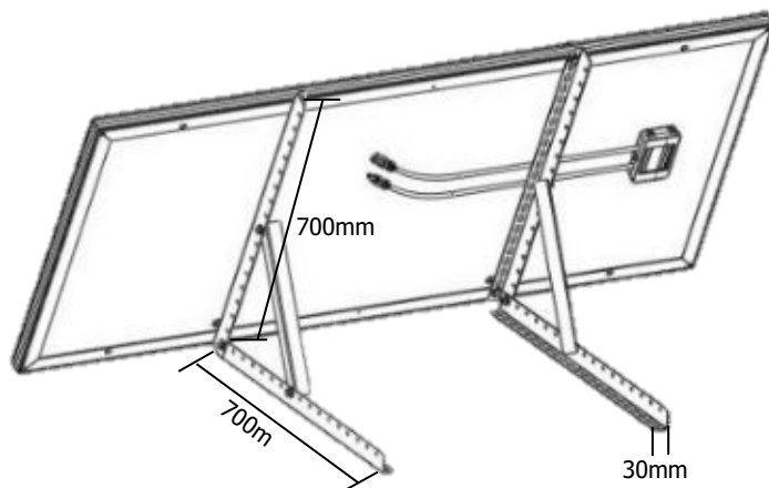
UNIFIX 150 B
