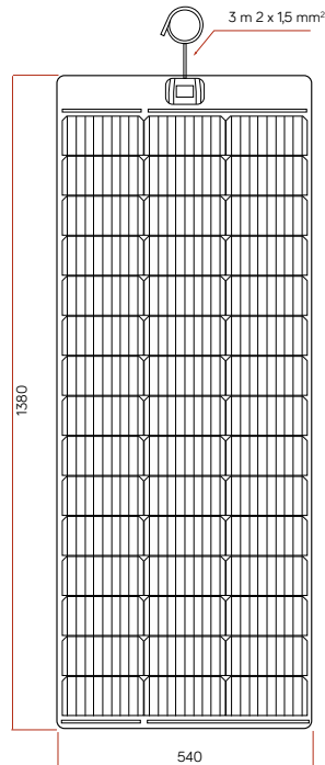
PERCFLEX145/ PERCFLEX145N
