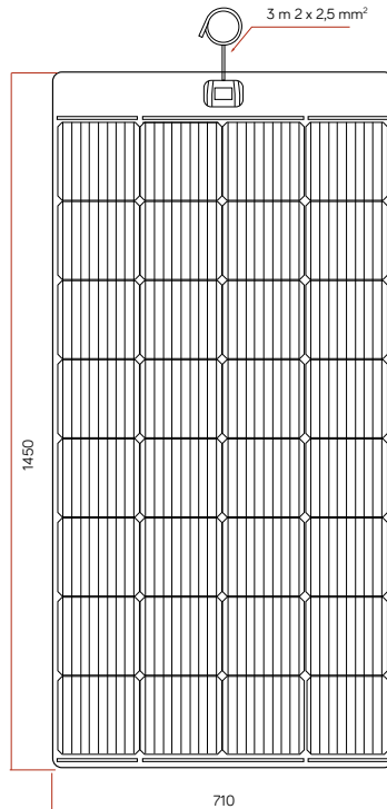
PERCFLEX210/ PERCFLEX210N
