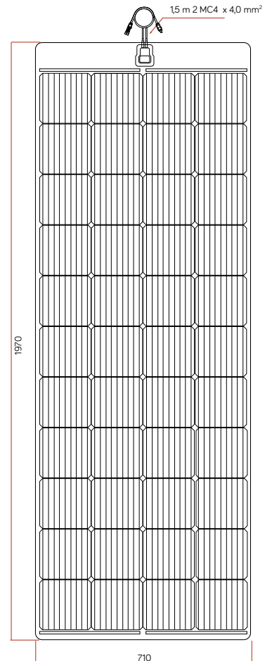
PERCFLEX280/ PERCFLEX280N
